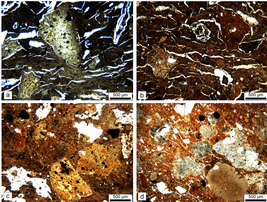
Fig. 11. Photomicrographs of thin sections taken from Belle-Plaine and Sainte-Claire (Plane-Polarized Light – PPL): Grog tempered sherds: (a) BP-47; (b) BP-47; (c) SC-27; (d) sandy matrix mainly with volcanic lithoclasts and isolated volcanic minerals SC-79.
