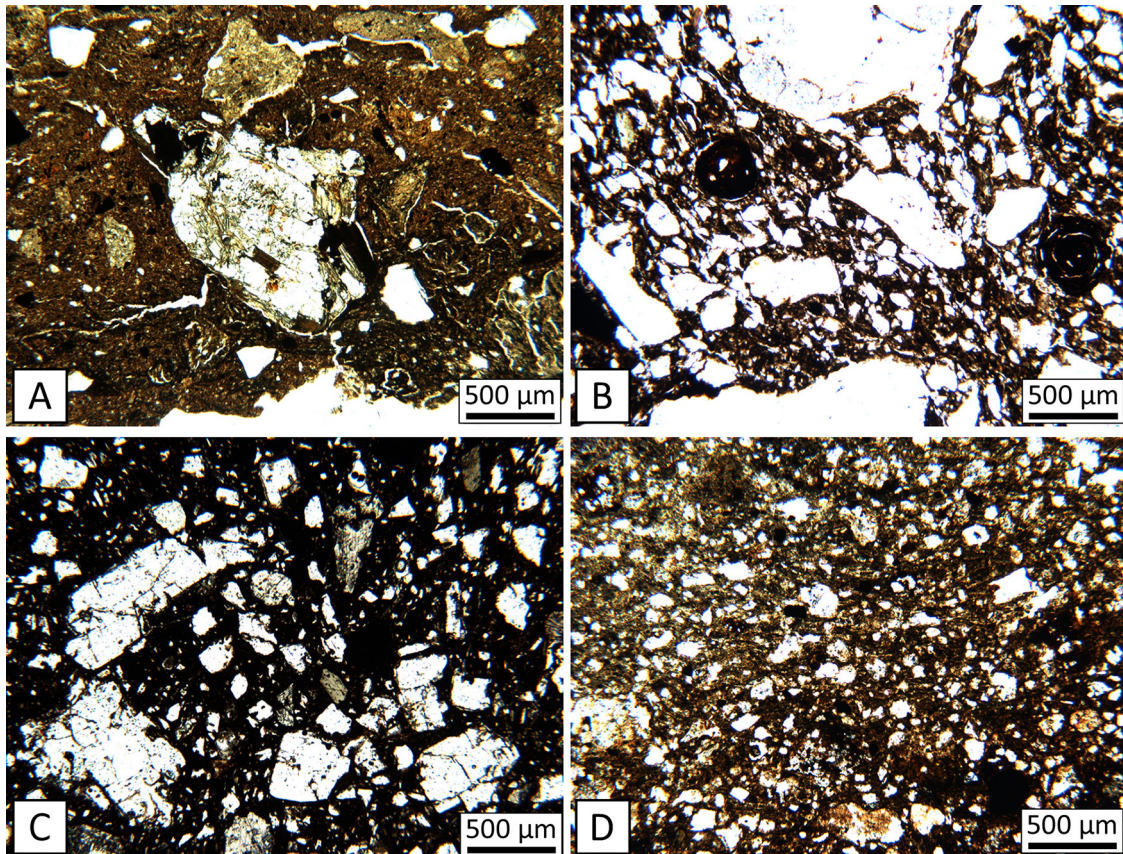
Fig. 7. Photomicrographs of thin sections showing minerals and lithoclasts from the discussed sites and comparatives ones (Plane-Polarized Light – PPL). A. Isolated weathered lithoclast (Cayenne, Perle-Noire, PN-212). B. Numerous pristine or poorly weathered lithoclasts (St-Martin, Grand Case, BK77-114). C. Volcanic sand (Capesterre-Belle-Eau, PR-5). D. Weathered small lithoclasts (Capesterre-Belle-Eau, PR-132).
