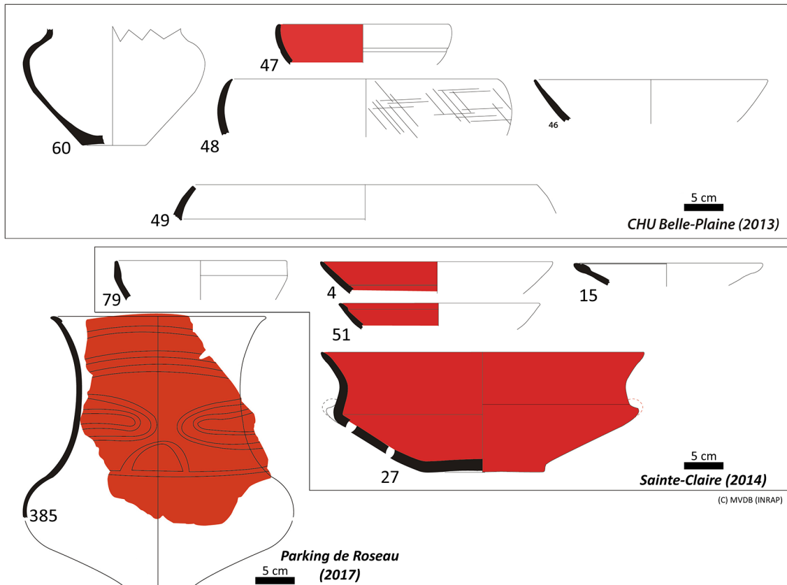
Fig. 4. Drawings of sampled vessels (Les Abymes, Goyave) and, from Parking de Roseau, reconstruction drawing of the Troumassoid vessel PR-385 (Capesterre-Belle-Eau).
