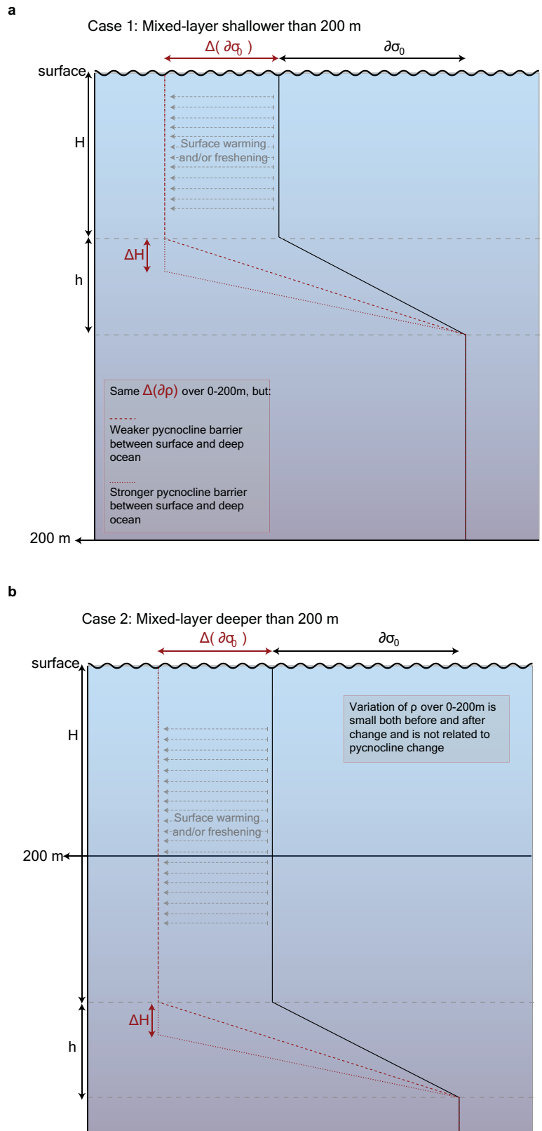
Extended Data Fig. 1 | Trends associated with the vertical structure of the upper ocean. a, b , Schematics showing idealized density profiles in the upper ocean for the cases in which the mixed layer and pycnocline are shallower (a) and deeper (b) than 200 m. The black line shows the typical shape of the density profile with a total density increase of \partial\rho across the pycnocline (thickness h )
