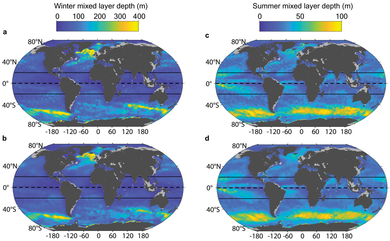
Extended Data Fig. 3 | Impact of linear-regression choices on mean mixed layer. a–d , Winter ( a, b ) and summer ( c, d ) mean mixed-layer depth computed using slightly different linear-regression models: Choice 1 ( a, c ; covariance
