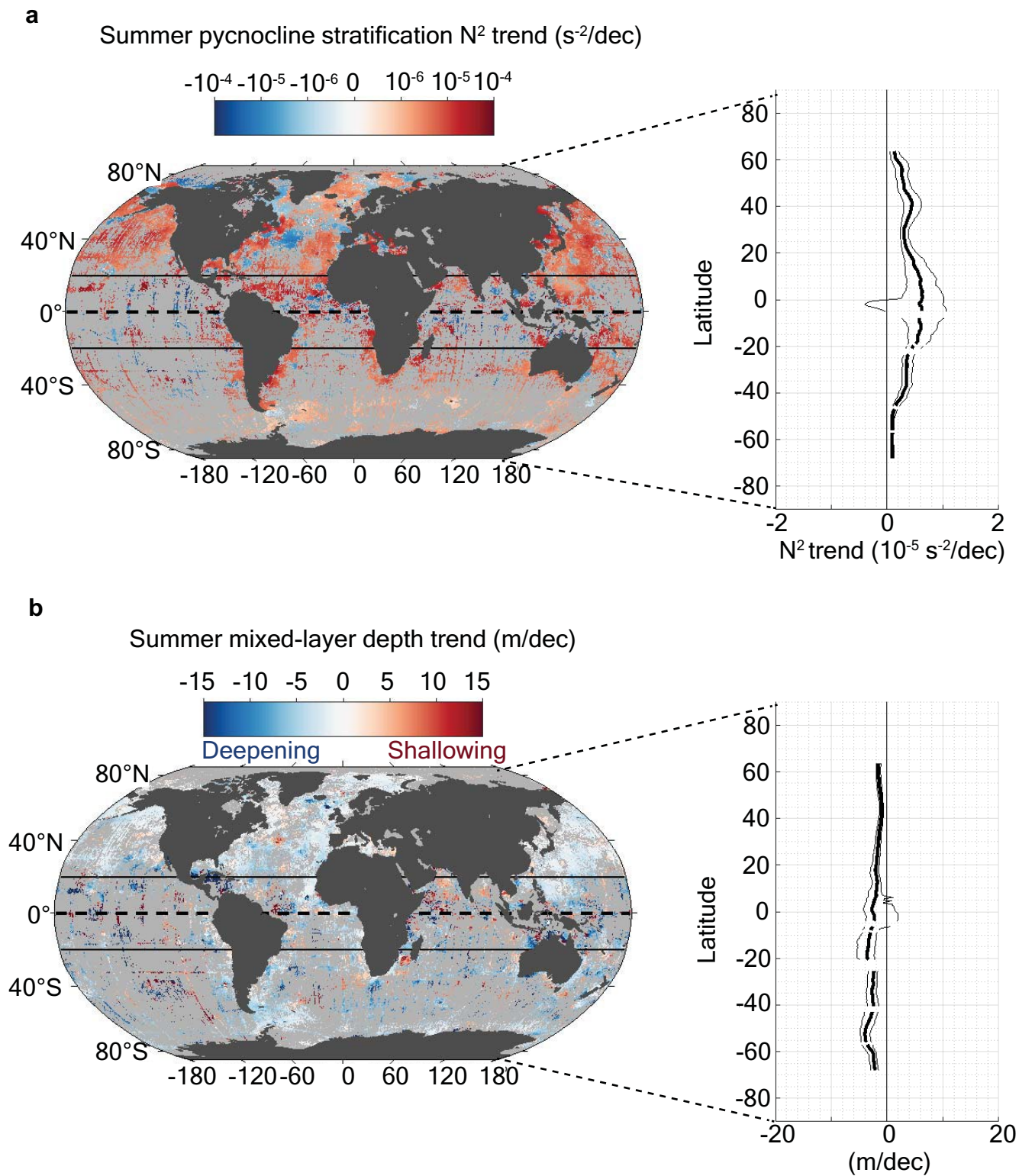
Extended Data Fig. 9 | 1970–2018 trends in summer pycnocline stratification and mixed-layer depth when using only ship-based profiles (removing all Argo and MEOP programme observations). a. Map of the 1970–2018 summer pycnocline stratification trend ( N^2 trend, in s^{-2} dec^{-1} ) along with the zonal-median value: median (thick black line) and 33th–66th
