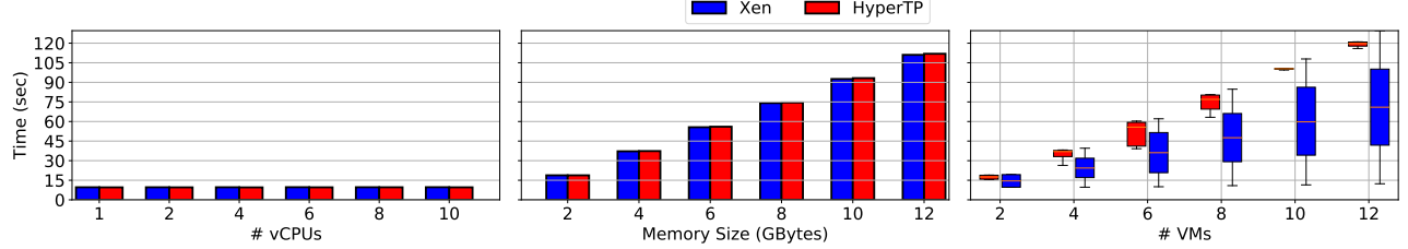
Figure 9: Total migration time in MigrationTP for Xen→KVM and Xen.
