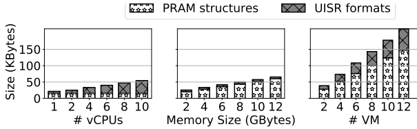
Figure 14: UISR memory size of InPlaceTP and MigrationTP .
