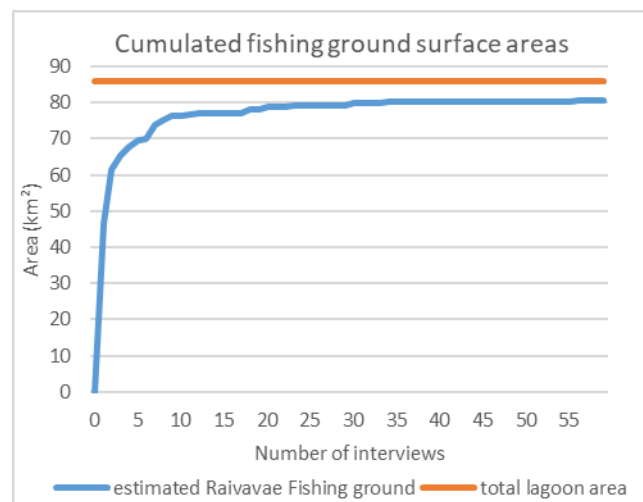
Figure 5. Cumulated fishing ground surface areas as a function of the number of interviews. It reaches an asymptote at 81 \text{km}^2 . The total lagoon surface area, reaching 86 \text{km}^2 , is displayed for comparison purpose.
