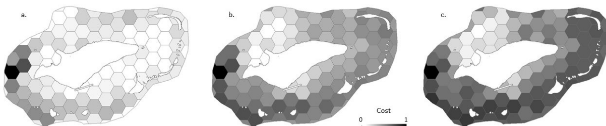
Figure 7. Maps of opportunity costs to fishers (unitless, from 0 to 1), calculated as fisheries modulated by ciguatera (see [Eq. (6)]) with different relative weights of ciguatera: a. relative ciguatera weight a = 0 (only fisheries as a cost); b. a = 0.5 ; c. a = 1 . In each case, values are normalised by the maximal value.
