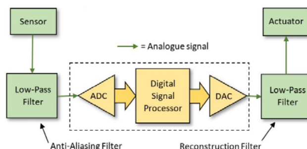
Fig. 3 The process of applying filter to the digital signals [23]
