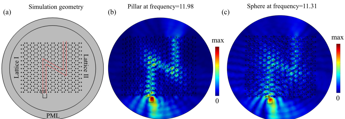
FIG. 5. (a) Schematic view of the numerical model: The phonic crystal plates consist of two lattices (as in Fig. 4) with a zigzag interface path (limited by the red lines); a finite antisymmetric Lamb wave source is excited along the white line segment (at the bottom exit of the zigzag path); a perfect marched layer (PML) is applied to surround the phonic crystal plates to avoid any wave reflection. The topologically protected edge state is excited by an antisymmetric Lamb wave at \Omega a = 11.98 for the pillar resonator (b) and at \Omega a = 11.31 for the sphere resonator (c) with a backscattering-immune property. The color bars show the amplitude of the displacement u_z .
