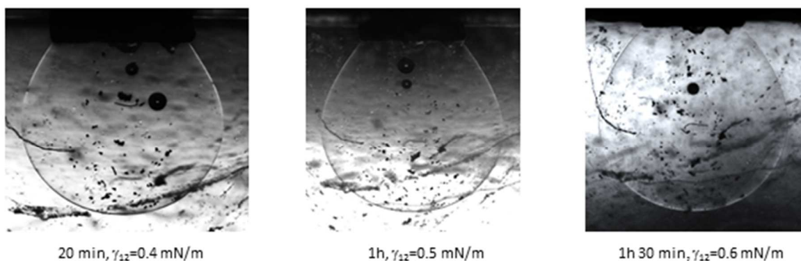
Figure 5: Experimental pendant drops of mPE in miPP at 200°C as a function of time.
