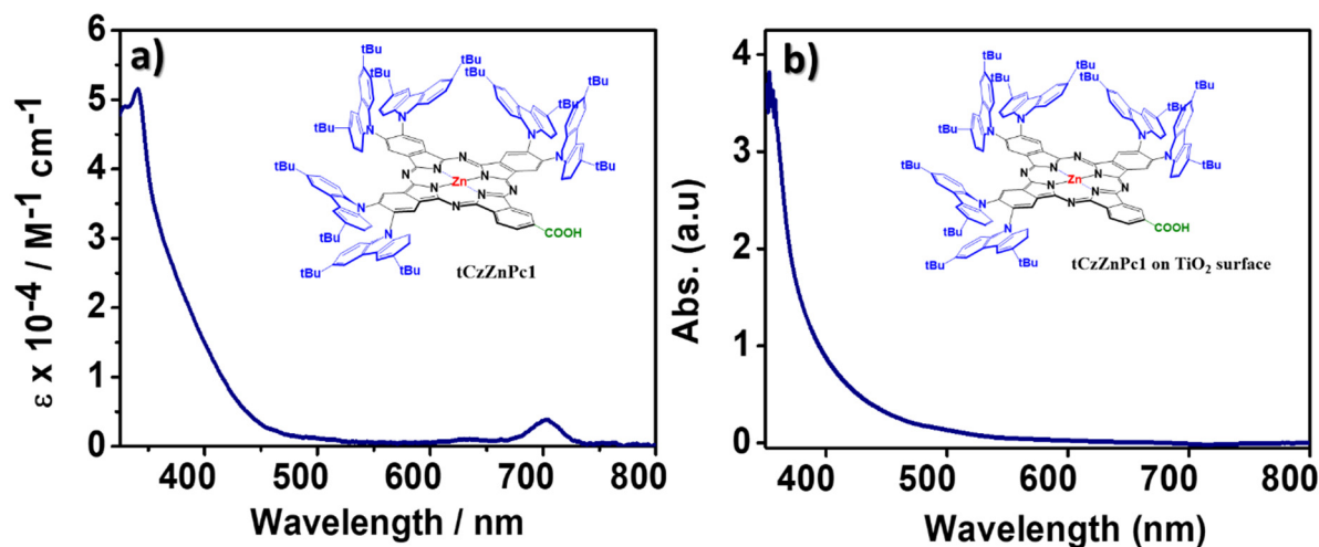
Figure 4. (a) Absorption in solution tCzZnPc1 (THF, 25 °C, 10^{-5} M), and (b) after adsorption on a 4 \mu m-thick transparent TiO 2 mesoporous electrode.
