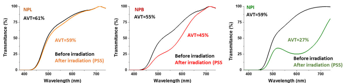
Supplementary Figure 24: Variation of the Average Visible Transmission of semi-transparent photochromic solar cells before irradiation and after light soaking (PSS reached under standard irradiation conditions).
