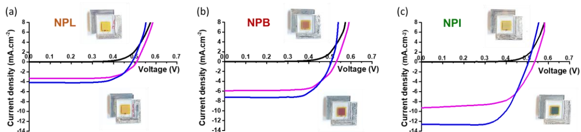
Figure 4 : Current-voltage characteristics of representative opaque photochromic solar cells registered in the dark (black line), after 15 seconds under irradiation (magenta line) and after few minutes of irradiation at the photo-stationary state (blue line) for (a) NPL , (b) NPB and (c) NPI . Insets show of the DSSCs before irradiation (top) and after full coloration under irradiation (bottom).
