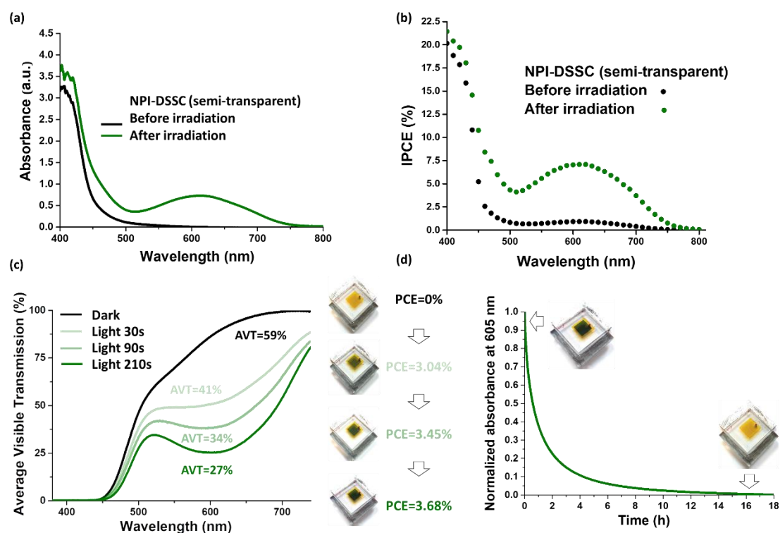
Figure 5: (a) UV-Vis spectrum of a complete semi-transparent NPI based solar cell (13 \mu\text{m} -thick \text{TiO}_2 ) before (black line, yellow solar cell) and after irradiation (green lines, green solar cells), IPCE spectrum of an NPI -based transparent solar cell before irradiation (black dots) and at the PSS after activation under irradiation (green dots). (c) Evolution of the Average Visible Transmission (AVT, measured between 380 and 740 nm) and PCE of a semi-transparent NPI -based solar cell as a function of light exposure time (standard irradiation conditions). (d) Bleaching curve registered at \lambda_{\text{max}} of a complete semi-transparent NPI based solar cell and picture of the cell before and after decolouration.
