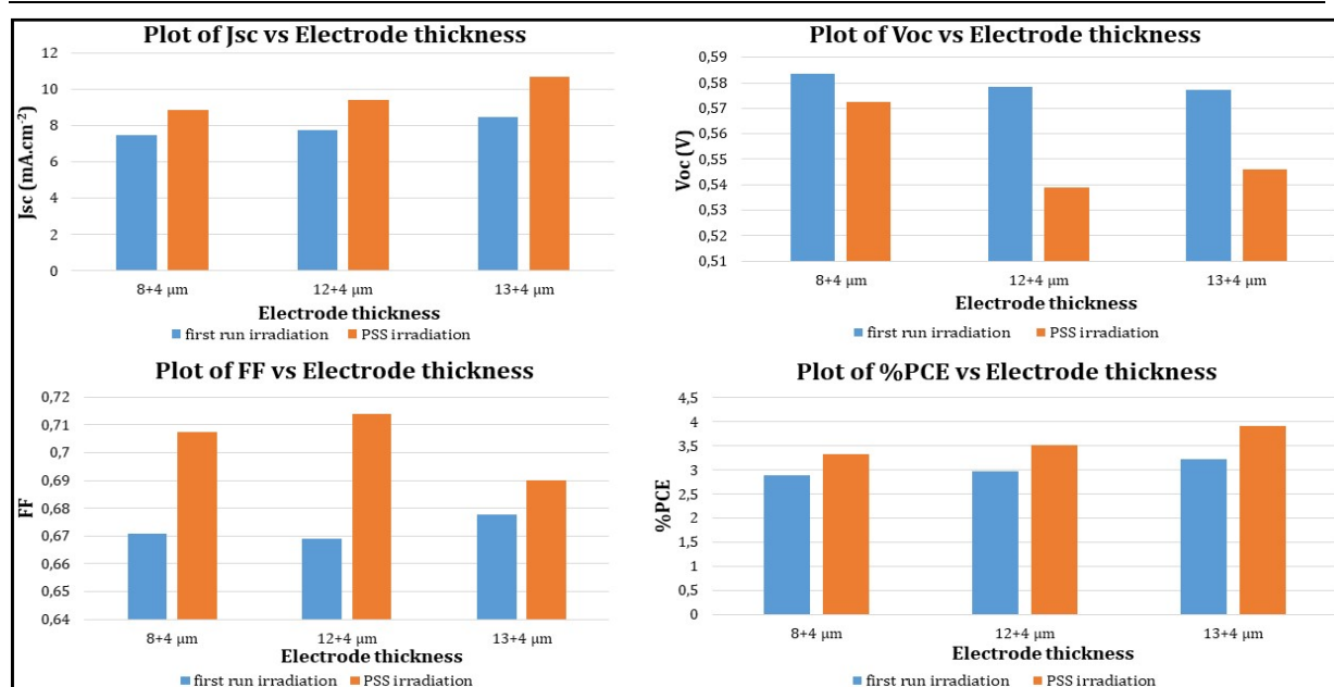
Supplementary Figure 21: Effect of electrode thickness on J_{sc} , V_{oc} , FF, and PCE for NPI-based opaque cells.
