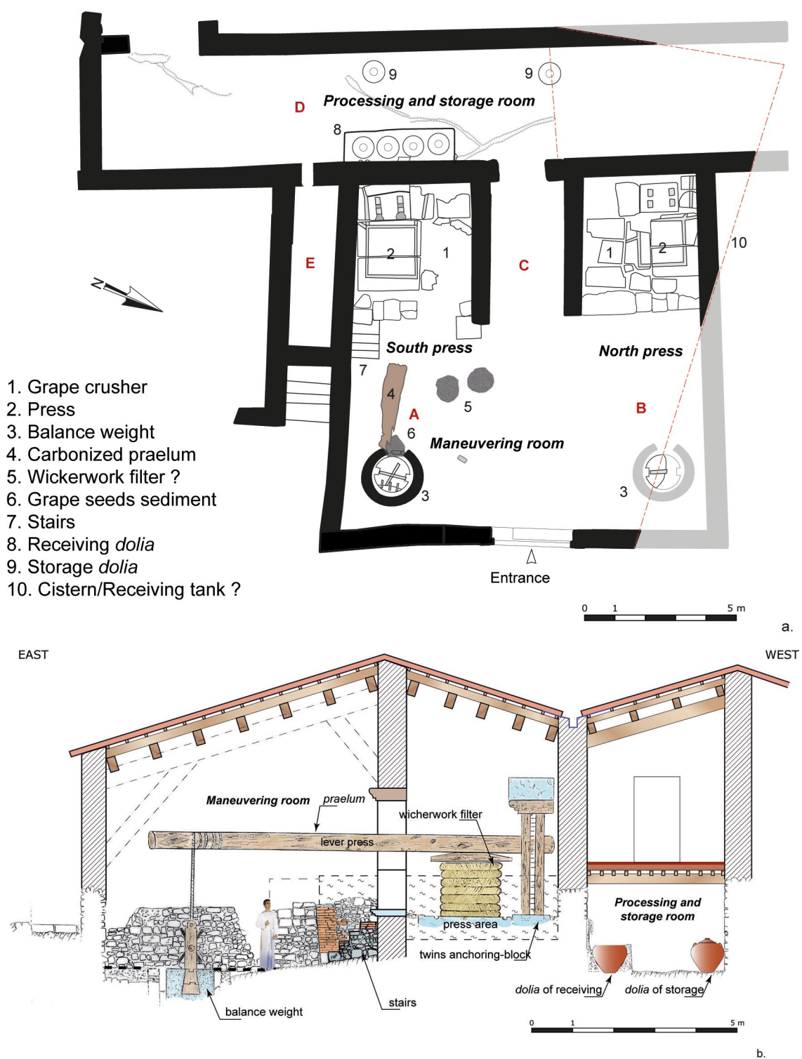
Fig. 2: Remains of winery at Rirha: (a) Explanatory ground-plan of production facility; (b) 2D hypothetical reconstructions of the southerly press.
