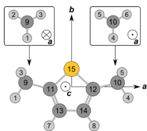
Figure 2 The molecular geometry of DMTP calculated at the MP2/cc-pVTZ level of theory given in its principal axes of inertia. The direction of the axes into and out of the paper plane is indicated by an encircled cross or dot, respectively.
