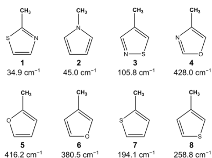
Figure 1 Barriers to internal rotation of some monomethyl unsaturated heterocyclic five-membered rings.
