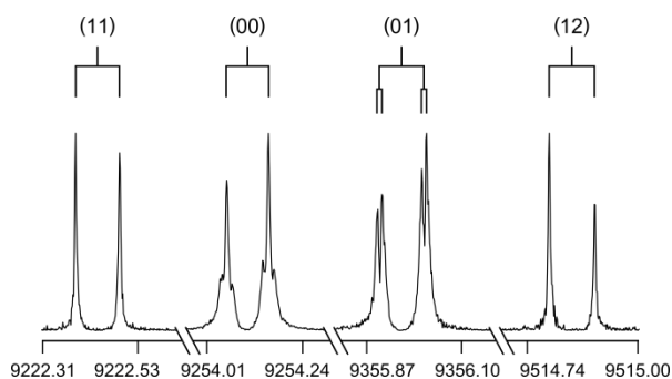
Figure 3 Typical spectra of the fur torsional species (00), (01), (11), and (12) of the 3_{21} \leftarrow 3_{12} transition of DMTP (in MHz). The experimental resolution is 2 kHz, the typical line width 10 kHz (FWHM). The larger splittings indicated by brackets are due to the Doppler effect; the smaller brackets indicate splittings of unknown origin. For these spectra, 21 – 614 decays were co-added. The intensities are normalized. An energy level diagram to illustrate the splitting is given in Fig. S-F4 in the SI.
