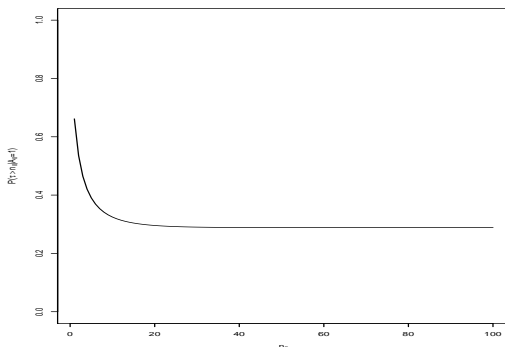
Figure 4: Numerical computation of the probability \mathbb{P}(\tau > n_0 \mid A_0 = 1) of obtaining a sample of size at least n_0 starting from 1 coupon at time 0, with c = 3 and for n_0 varying between 1 and 100.
