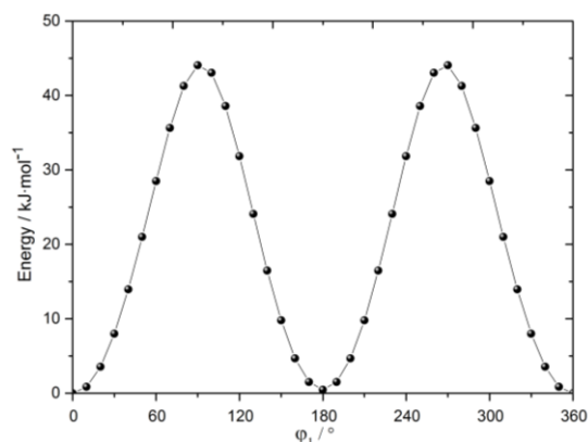
Figure 2. The potential energy curve of MFF obtained by rotating the formyl group around the C 2 –C 7 bond, i.e., by varying the dihedral angle \varphi_1 = \angle(O_1, C_2, C_7, H_9) in a grid of 10° at the MP2/6-311++G(d,p) level of theory. Two stable C s conformers were found at \varphi_1 = 0^\circ ( cis ) and 180^\circ ( trans ) differ by only 0.48 kJ·mol -1 in energy. The relative energies are given with respect to the lowest energy conformation ( cis -MFF: E = -381.7235146 Hartree).
