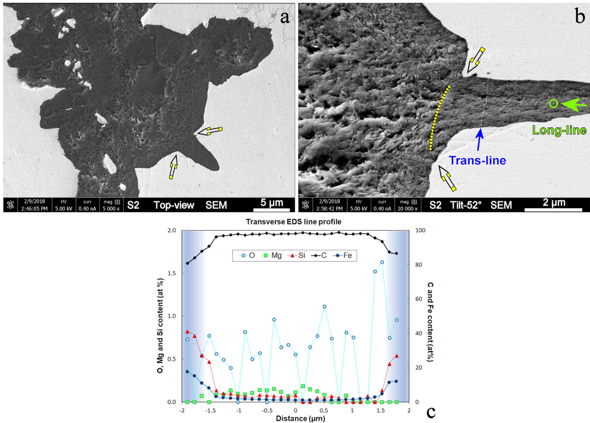
Fig. 4. (a) SEM micrograph (top view) of a degenerate graphite spheroid (S2) with outgrowths. Open arrows indicate the change of surface features; (b) Higher magnification tilted view (52°) of the region of interest; (c) EDS line profiles, registered along transverse (Trans-line) direction of the outgrowth (see corresponding wt% line profile in Suppl-Fig. 1). (A colour version of this figure can be viewed online.)
