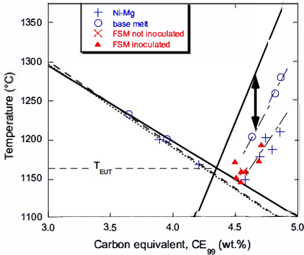
Fig. 2 Values of the first arrest on the cooling curves as function of CE_{99} for laboratory not inoculated alloys [6] and FSM treated industrial alloys [9] with silicon content between 2.40 and 2.84 wt pct. The solid lines are the austenite and graphite liquidus (Eqs. [1] and [2] at 2.6 wt pct Si); their intersection at CE_{99} = 4.34 wt pct represents the eutectic point in the Fe-C isopleth section. Dotted and short dashed lines show the austenite liquidus according to Eqs. [5] and [6], respectively. The two dashed lines have been drawn through the available data for hypereutectic base melts and Mg treated alloys, respectively. The double arrow shows how is defined the undercooling \Delta T_L^{gra} with respect to graphite liquidus.
