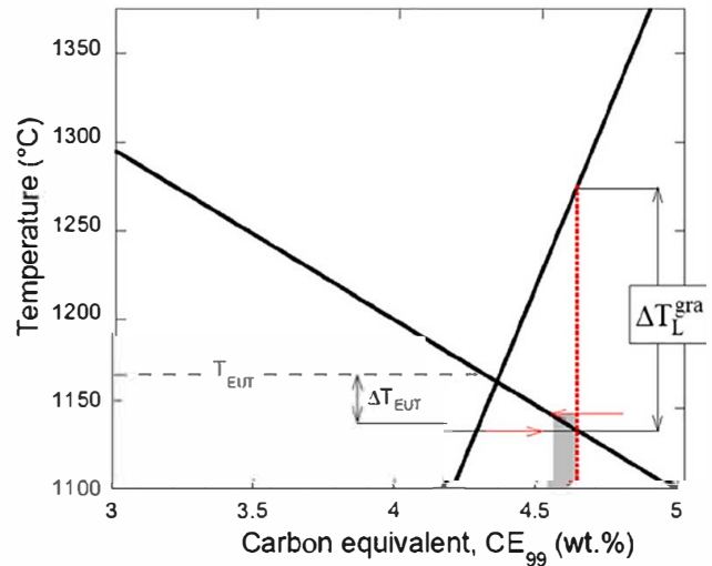
Fig. 10 Schematic showing how to define highly hypereutectic alloys to the right of the vertical dotted line from mildly hypereutectic alloys to the left. The grayed area is the transition zone, see text. The bold solid lines are the austenite and graphite liquidus (Eqs. [1] and [2]) calculated at 2.6 wt pct Si.
