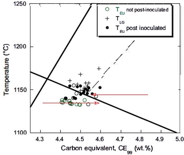
Fig. 7 Values of T_{LG} (plus signs) and T_{EU} (circles and dots) as function of CE_{99} for industrial alloys with silicon content between 2.03 and 2.42 wt pct Si. The bold solid lines are the austenite and graphite liquidus (Eqs. [1] and [2]) calculated at 2.18 wt pct Si, 0.47 wt pct Mn, and 0.39 wt pct Cu. The dashed line is at the same undercooling \Delta T_{E}^{gr} as the one for spheroidized alloys in Fig. 2. The red arrows are located at the same eutectic undercoolings as in Fig. 3.
