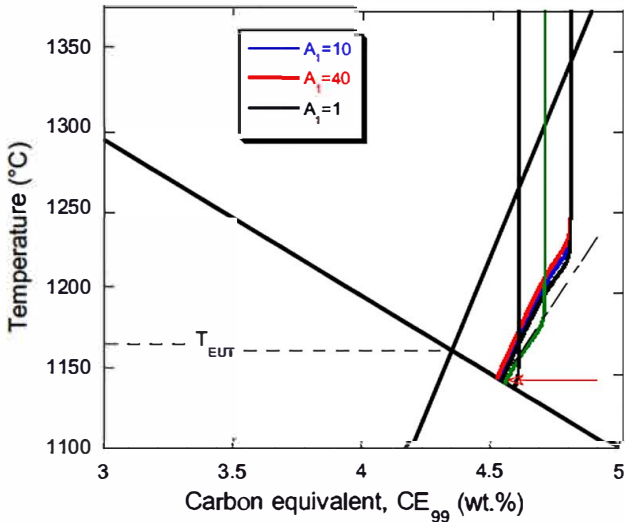
Fig. 9 Solidification path of hypereutectic alloys shown in the CE_{99} -T plane. Calculations for CE_{99} = 4.8 wt pct were performed for three A_1 values, 1, 10, and 40 mm^3 K^{-1} . Calculations for CE_{99} at 4.6 wt pct and 4.7 wt pct were carried out with A_1 = 1 mm^3 K^{-1} . The bold solid lines are the austenite and graphite liquidus (Eqs. [1] and [2]) calculated at 2.6 wt pct Si. The dashed line represents the thermal arrest for Mg treated alloys as in Fig. 2.
