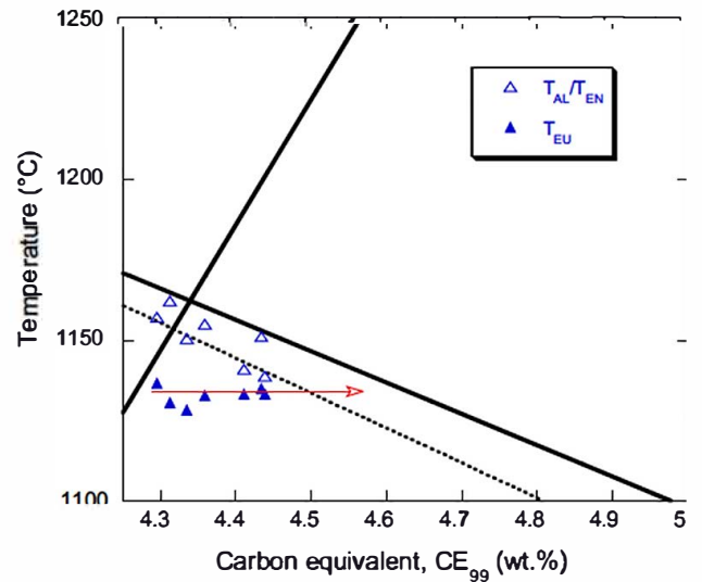
Fig. 4 Values of the T_{AL} or T_{EN} (open symbols) and of T_{EU} (solid symbols) arrests as function of CE_{99} for alloys with silicon content between 1.86 and 2.20 wt pct. [9] The bold solid lines are the austenite and graphite liquidus (Eqs. [1] and [2]) and the dotted line is the T_{AL,base} austenite liquidus (Eq. [5]), all calculated at 2.0 wt pct Si. The red arrow is located at the same eutectic undercooling as in Fig. 3, \Delta T_{EUT} = 28 °C.
