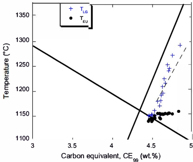
Fig. 5 Values of the T_{LG} (crosses) and T_{EU} (solid dots) arrests as function of CE_{99} for alloys with silicon content between 1.70 and 1.91 wt pct Si. The bold solid lines are the austenite and graphite liquidus (Eqs. [1] and [2]) calculated at 1.8 wt pct Si, 0.19 wt pct Mn and 0.07 wt pct Cu. The dashed line is positioned at the same undercooling with respect to the graphite liquidus as the one for base melts in Fig. 2.
