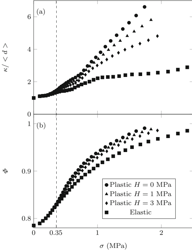
Fig. 3 Mean value of maximum curvature \kappa of the particles normalised by their mean diameter \langle d \rangle (a) and the packing fraction \Phi (b) as a function of the applied stress \sigma for elastic and elasto-plastic material behaviours
