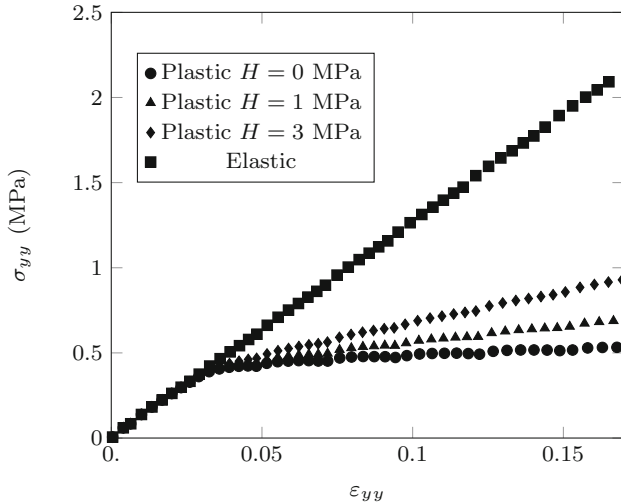
Fig. 1 Stress–strain diagrams for the single elastic and elasto-plastic (with several values of hardening) particles subjected to diametrical compression
