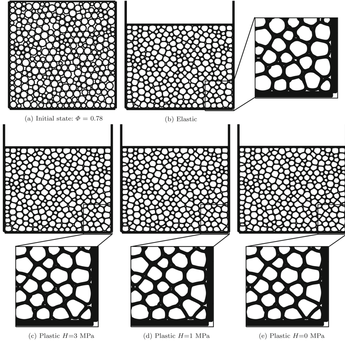
Fig. 2 A snapshot of the initial configuration (a); snapshots of the compacted packings of particles with elastic and elasto-plastic behaviours (with three values of the hardening parameter H ) at packing fraction of \Phi = 0.97 , and zoom on the particles inside a bottom right window of the deformed packings (b–e)
