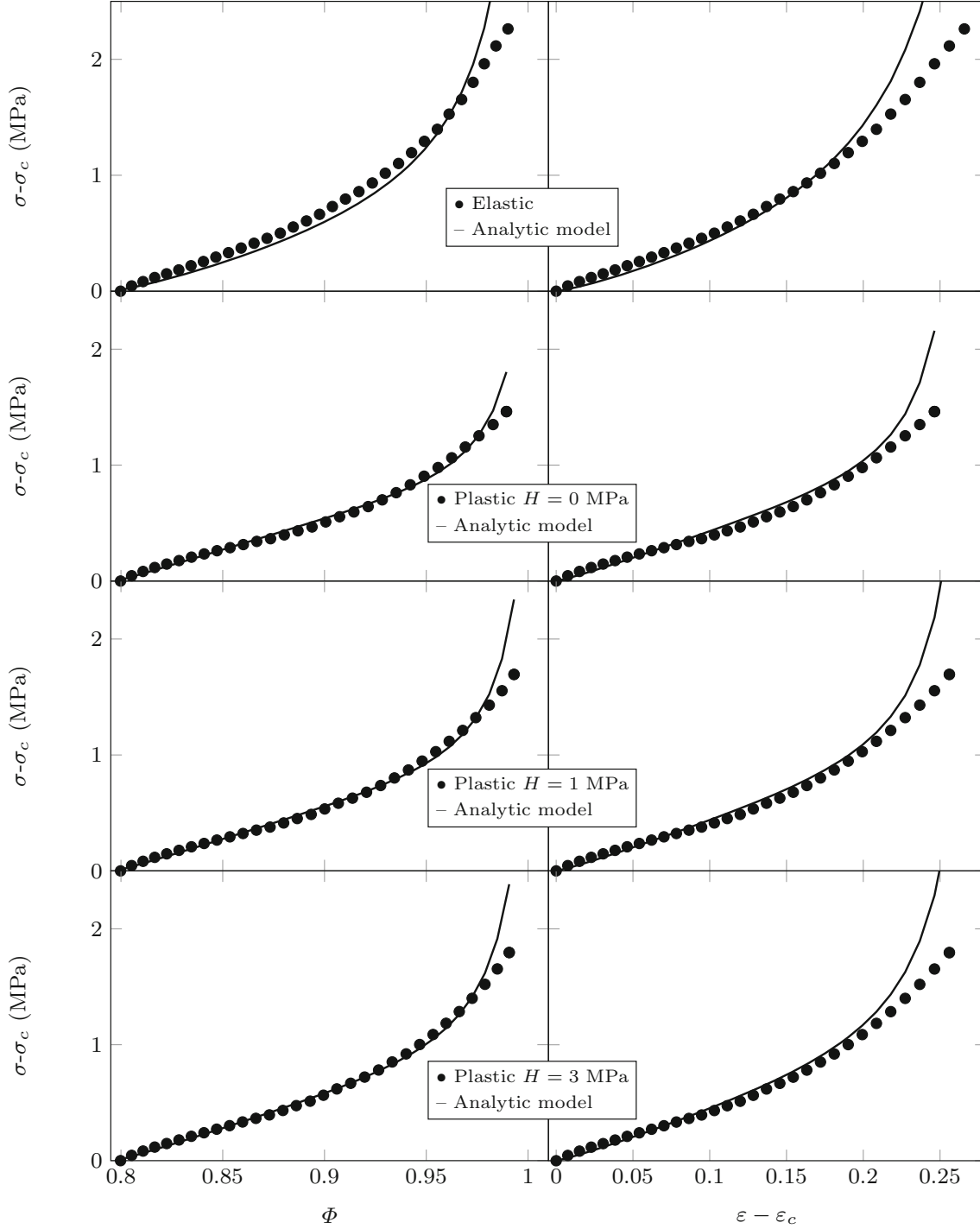
Fig. 4 Excess applied stress \sigma - \sigma_c as a function of packing fraction \Phi and excess strain \varepsilon - \varepsilon_c for elastic and elasto-plastic (with three values of hardening, H ) particles by MPM simulations. \sigma_c and \varepsilon_c correspond
