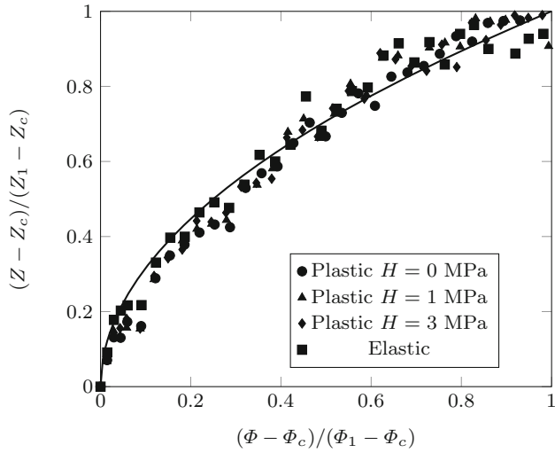
Fig. 5 Evolution of the excess mean coordination number Z - Z_c as a function of excess packing fraction \Phi - \Phi_c for elastic and elasto-plastic particles by MPM simulations. The solid line is power-law fit (\Phi - \Phi_c)^{0.5} ; see Eq. (17)
