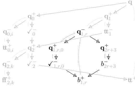
Figure 64: Events of |\alpha_{\mathbf{q}_1^+,1}| of Figure 61
