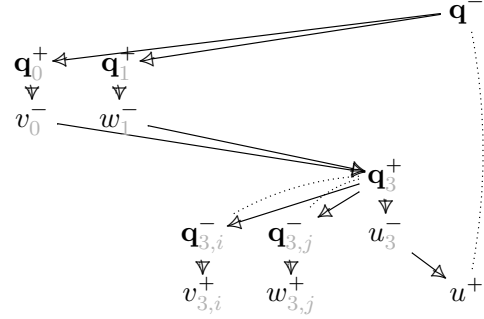
Figure 38: The strategy \text{plet}_{\mathbb{X},\mathbb{Y}}
