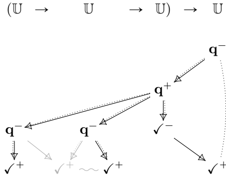
Figure 43: \lambda f^{\mathbb{U} \rightarrow \mathbb{U} \rightarrow \mathbb{U}}. \mathbf{newref} \ r := 0 \ \mathbf{in} \quad f \ (r := 1) \quad (\mathbf{skip} \ \otimes \ (\mathbf{assume} \ !r))
