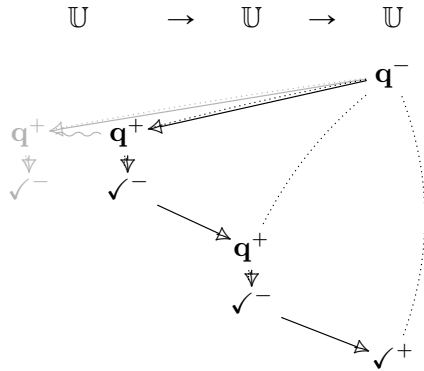
Figure 42: \lambda x^{\mathbb{U}} y^{\mathbb{U}}. \mathbf{newref} \ r := 0 \ \mathbf{in} \quad \mathbf{assume} \ (\mathbf{iszero} \ !r); \ x; \ r := \mathbf{tt} \quad \parallel \ \mathbf{assume} \ (\mathbf{not} \ (\mathbf{iszero} \ !r)); \ y
