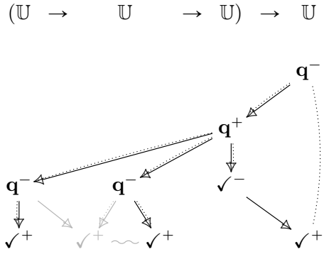
Figure 43: \lambda f^{\mathbb{U} \rightarrow \mathbb{U} \rightarrow \mathbb{U}}. \text{newref } r := 0 \text{ in} \quad f (r := 1) \quad (\text{skip } \odot (\text{assume !r}))
