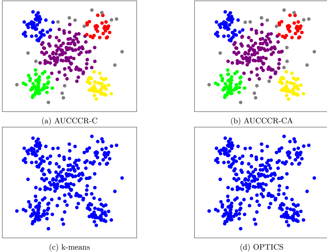
Figure 5: Clusters found in Gaussians Star
