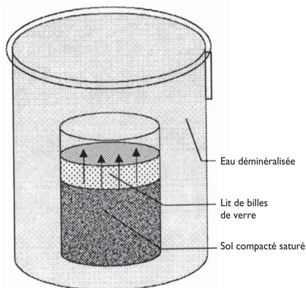
Figure 1 : Compact Granular Leach Test: principe
