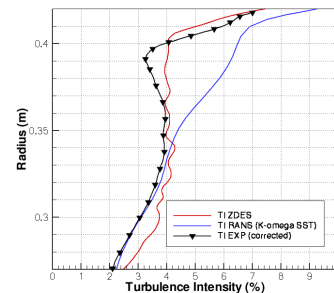
Figure 9. Comparison of turbulence intensity profiles assessed by ZDES, RANS and corrected experiment.
