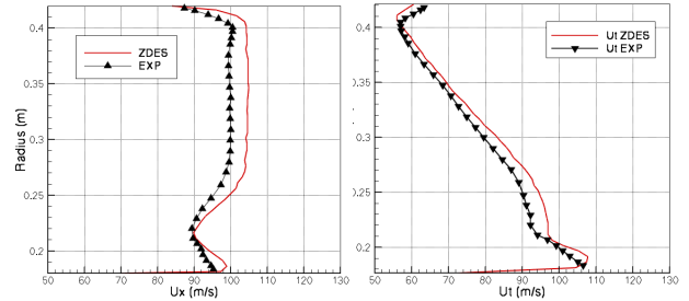
Figure 7. ZDES vs. experiment mean velocity profiles for axial (left) and tangential (right) components.
