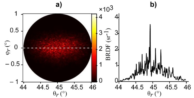
Figure 2. BRDF measurement with ConDOR. Left: single shot image. Right: cross-section along the dashed line shown on the left.
