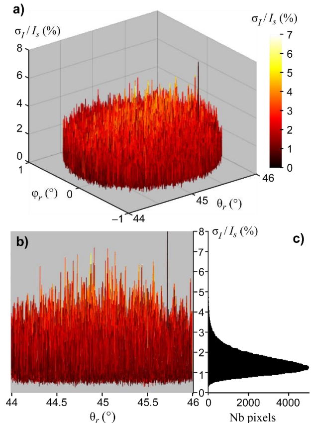
Figure 3. Standard deviation of the relative shot-to-shot fluctuations of the detected signal. a) 3D view and b) side view showing the values of the standard deviation obtained on each pixel of the detector, calculated from 100 images. c) Histogram of the standard deviation values.
