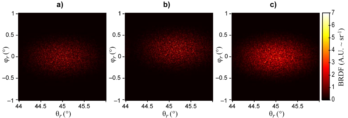
Figure 6 – Speckle patterns simulated under different illumination conditions: (a) the light source is a point on axis, leading to an image centered on the CCD detector; (b) the light source is a point shifted off-axis by 0.17^\circ in both \theta_i and \phi_i directions, leading to the exact same speckle pattern but tilted by the same angular amount. (c) the light source is a square with uniform illumination and 100\mu\text{m} diagonal size, equivalent to 0.014^\circ in angular size.
