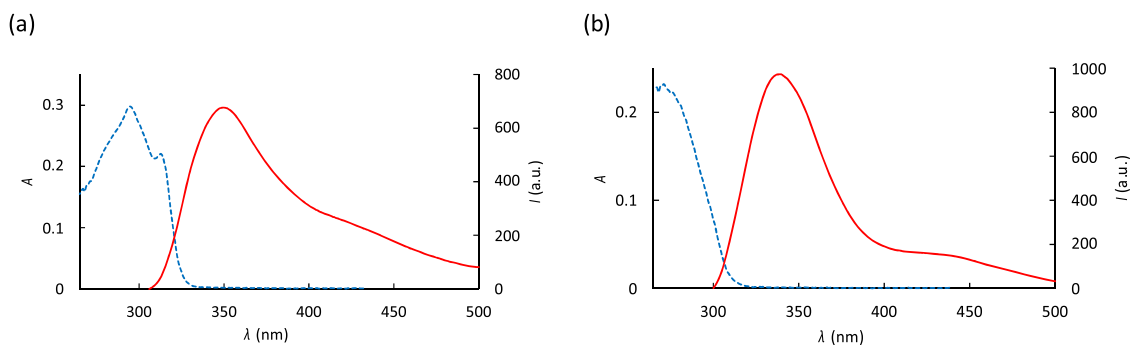
Figure 3. Absorption spectra (in blue) and emission spectra (in red, \lambda_{\text{exc}} = 290 nm): (a) hemicryptophane 2 (3.2 \mu\text{M} ) and (b) hemicryptophane 3 (4.7 \mu\text{M} ) in solution in DMSO + 2% H 2 O at 298 K.
