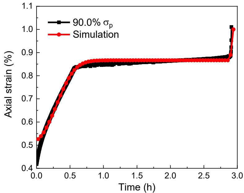
389 Figure 17 Comparison between experimental (black curve) and numerical (red curve) creep strain curve of 390 Lanhélin granite 391 392
