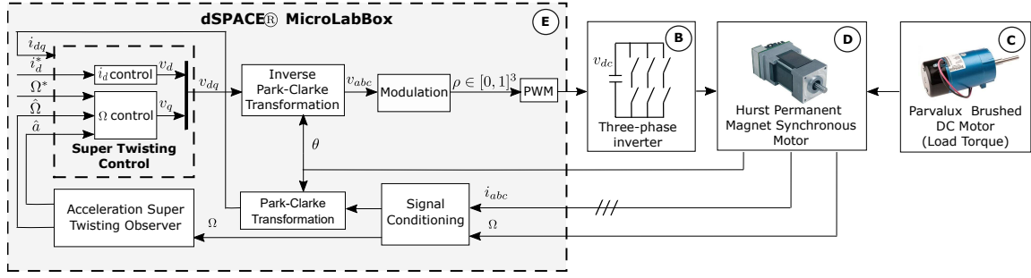
Fig. 2: Control Scheme
