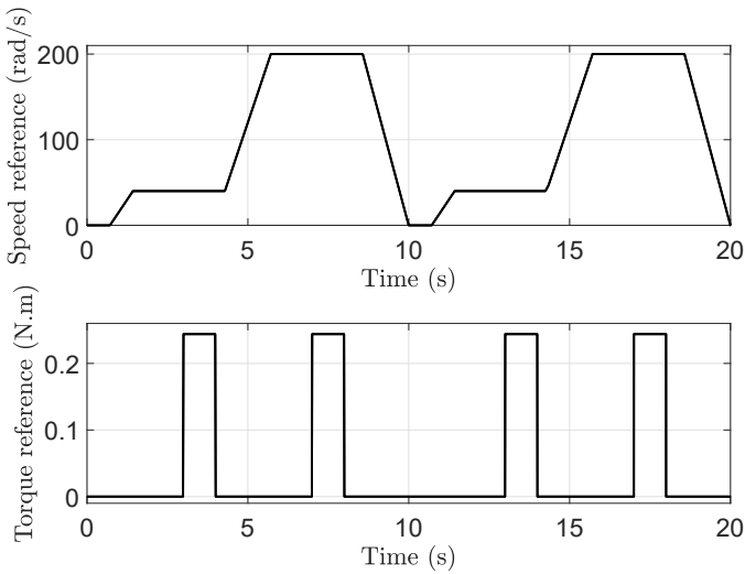
Fig. 4: Industrial test trajectories
