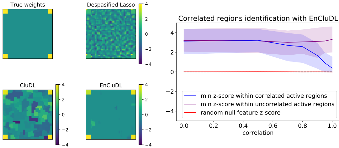
Figure 11: Impact of correlation when trying to identify two correlated regions. Left: True weight map, and z-scores estimated by Desparsified Lasso, CluDL and EnCluDL, obtained for \rho = 0.9 . Desparsified Lasso cannot handle the extreme short-range correlation that occurs within each predictive region and only identifies one feature in each. CluDL and EnCluDL benefit from the clustering, as they identify all the features for every predictive regions. We can also observe that EnCluDL improves upon CluDL thanks to the smoothing effect produced by ensembling. Focusing on the EnCluDL solution, we can see that the z-score of the upper left active region is a bit lower than for the other active regions. This is due to the high correlation between the upper left and bottom right regions. Right: Summary of the results of the second simulation. When the correlation increases the minimum z-score within the correlated active regions decreases. The minimum z-score between the two uncorrelated regions is used as a control. We also plot the z-score of a random non-predictive feature, we notice that due to the ensembling step of EnCluDL, the empirical confidence intervals are much thinner than in Fig. 10. We observe that for a correlation lower than 0.8 the deviation is limited and it is possible to identify the two correlated predictive regions. For a correlation larger than 0.9 the deviation becomes large and recovering the two correlated regions becomes impossible.
