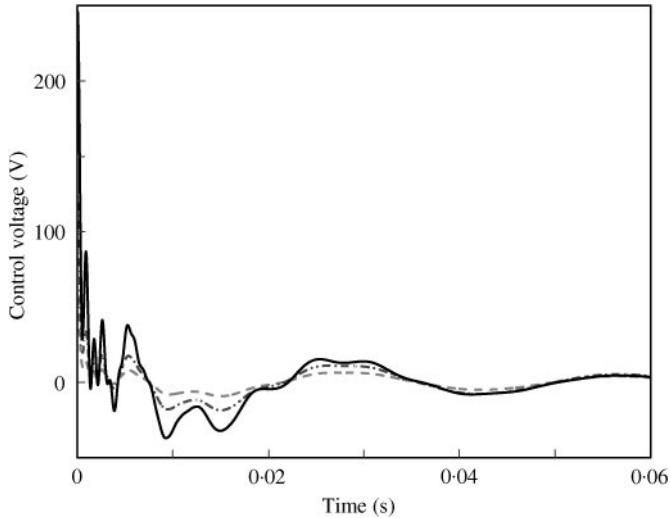
Figure 14. Control voltages imposed to the piezoelectric actuator for three velocity feedback control gains. K_d values: --- , 137; \cdot\cdot\cdot , 302; — , 605.
