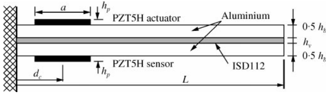
Figure 2. Cantilever sandwich beam with bonded piezoelectric actuator and sensor.
