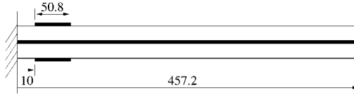
Figure 2. Cantilever sandwich beam with bonded actuators (dimensions in mm).
