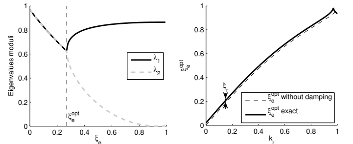
Figure 6. (left) Moduli of eigenvalues of \mathbf{A}^{\text{SSDI}}\mathbf{B} for k_r = 0.2 and \xi_r = 2\% ; (right) optimal electrical damping \xi_e^{\text{opt}} as functions of k_r , which mechanical damping
