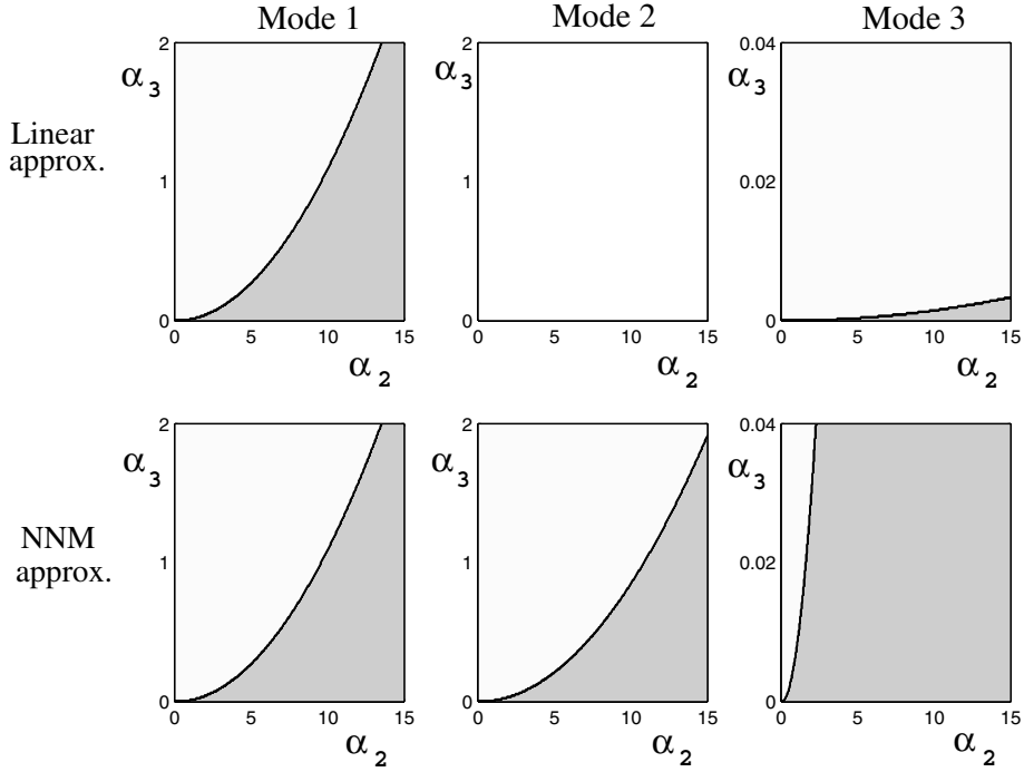
Fig. 1. Hardening and softening regions for the linear beam resting on a non-linear elastic foundation. White: hardening behaviour. Gray: softening behaviour.
