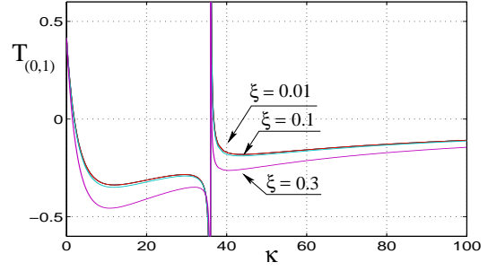
Figure 7. Type of non-linearity for mode (0,1) versus the aspect ratio \kappa of a shallow spherical shell. Increasing values of damping for case of "proportional damping" ( \forall p = 1 \dots N, \xi_p = \xi ), are shown, with \xi = 0 and 0.01 (red), 0.1 (cyan) and 0.3 (violet).
