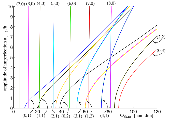
Figure 1. Non-dimensional natural frequencies \omega_{(k,n)} of the imperfect plate versus the amplitude of the imperfection having the shape of mode (0,1).
