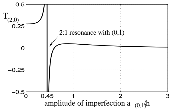
Figure 3. Type of non-linearity for mode (2,0) with an axisymmetric imperfection having the shape of mode (0,1).
