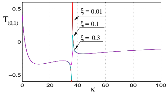
Figure 6. Type of non-linearity for mode (0,1) versus the aspect ratio \kappa of a shallow spherical shell. Increasing values of damping for case of "constant damping" ( \forall p = 1 \dots N, \xi_p = \xi / \omega_p ), are shown, with \xi = 0 and 0.01 (red), 0.1 (cyan) and 0.3 (violet).
