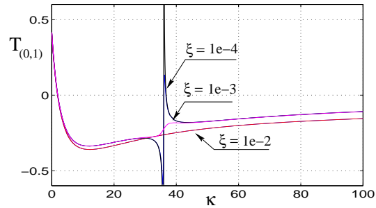
Figure 8. Type of non-linearity for mode (0,1) versus the aspect ratio \kappa of a shallow spherical shell. Increasing values of damping for case of "square damping" ( \forall p = 1 \dots N, \xi_p = \xi \omega_p ), are shown, with \xi = 0 and 1e-4 (black and blue, collapsed), 1e-3 (magenta) and 1e-2 (red).
