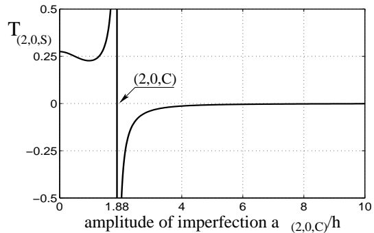
Figure 5. Type of non-linearity for mode (2,0,S) for an imperfection having the shape of mode (2,0,C).
