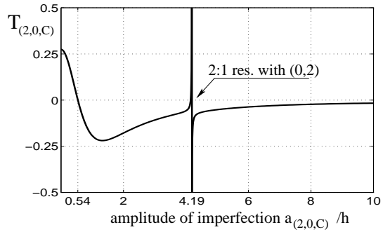
Figure 4. Type of non-linearity for mode (2,0,C) for an imperfection having the shape of mode (2,0,C).
