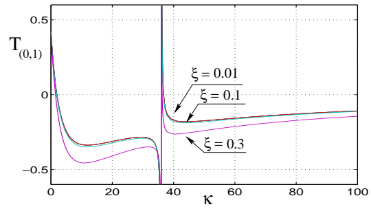
Figure 7. Type of non-linearity for mode (0,1) versus the aspect ratio \kappa of a shallow spherical shell. Increasing values of damping for case of "proportional damping" ( \forall p = 1 \dots N, \xi_p = \xi ), are shown, with \xi = 0 and 0.01 (red), 0.1 (cyan) and 0.3 (violet).
