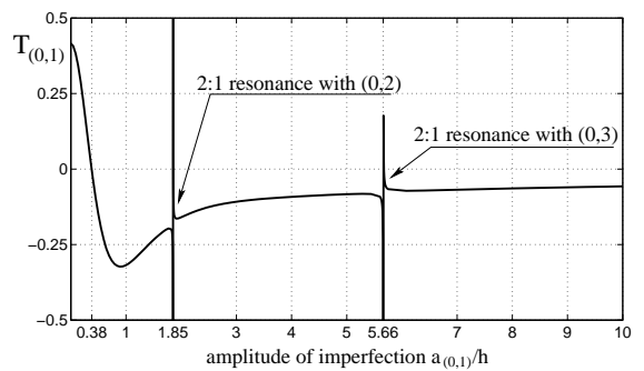
Figure 2. Type of non-linearity for mode (0,1) with an axisymmetric imperfection having the shape of mode (0,1).
