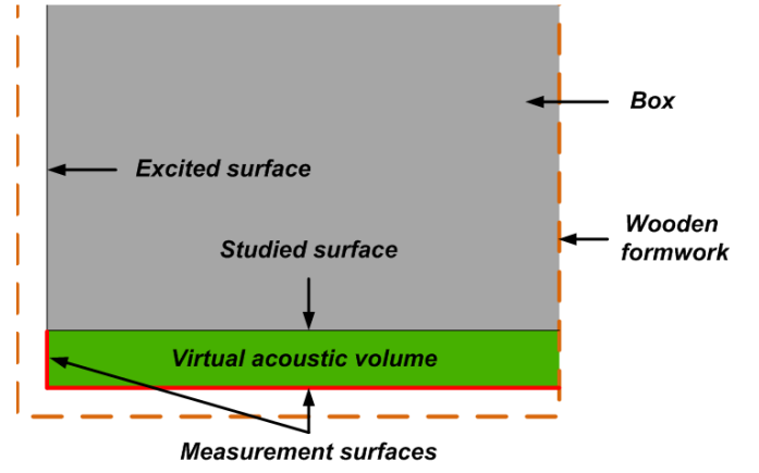
Fig.10 Definition of the virtual acoustic volume
