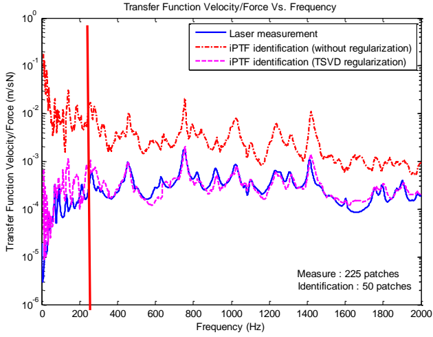
Fig.4 Identification of source velocity: (-) Reference (laser vibrometer), (-.-) iPTF identification without regularization, (-.-) iPTF identification with TSVD identification for 225 measurement patches and 50 identification patches
