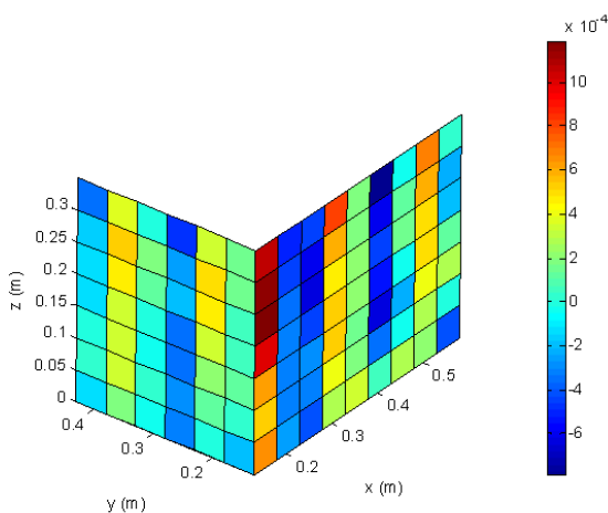
Fig.9 Source velocity field identified with the iPTF method for 105 identification patches at 1756Hz
