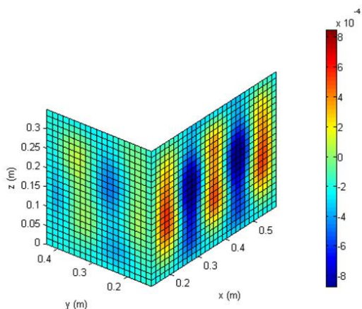
Fig.8 Source velocity field measured with a laser vibrometer at 1756Hz
