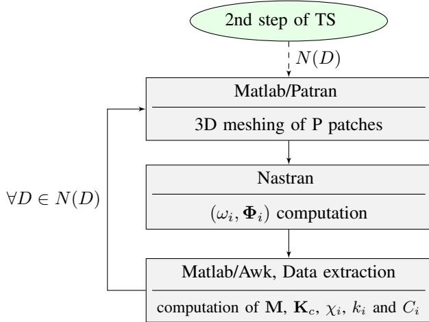
FIGURE 4. 2nd STEP OF THE TABU SEARCH
