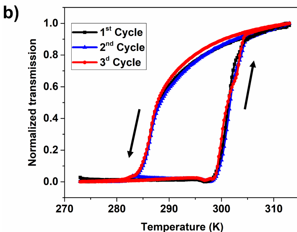
Figure 1. (a) Reproducibility of the SCO in four different single crystals of 1 . (b) Reproducibility of the SCO in a single crystal of 1 for three subsequent thermal cycles. All data were acquired at 1 \text{ K min}^{-1} . Heating and cooling are indicated by arrows.
