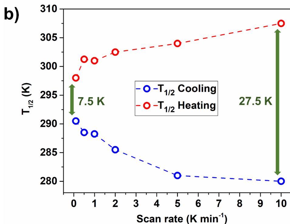
Figure 2. (a) Temperature scan-rate study (0.1–10 K min -1 ) of the spin transition (normalized optical transmission vs. temperature) in a single crystal of 1 . (b) Scan-rate dependence of the spin-transition temperatures in the heating and cooling modes.
