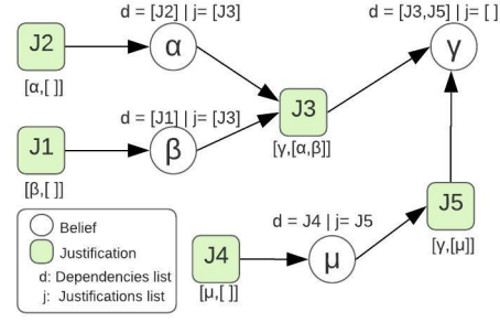
Fig. 1. Graph over the beliefs and justifications.
