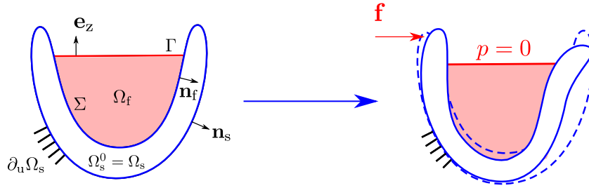
Figure 2: Hydroelastic problem description without pre-stress effect under a small amplitude harmonic load \mathbf{f} , with no gravity effect such that the pressure fluctuation is fixed as p = 0 on the free surface \Gamma .
