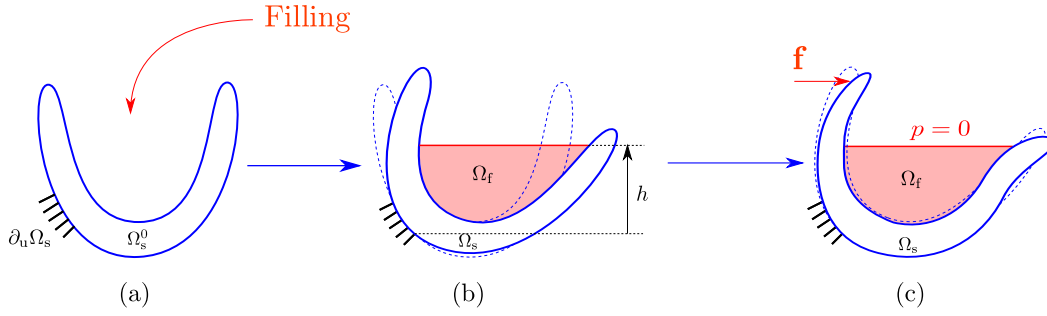
Figure 4: (a) Reference configuration without fluid; (b) current configuration for a given fluid height; (c) linearized vibration around a prestressed state under a small amplitude excitation \mathbf{f} .
