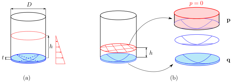
Figure 5: (a) Filling of a cylinder of diameter D = 357 mm with water \rho_f = 1000 kg.m -3 , rigid walls and an elastic bottom of thickness t = 0.357 mm made of plexiglas. The material parameters are the Young Modulus E = 5.47e9 Pa and a Poisson Ratio of 0.38 and the plexiglas density \rho_s = 1.38 kg.m -3 . The fluid height value is such that h \in [0, 250] mm; (b) Hydroelastic vibrations around the pre-stressed state for a given fluid height h .
