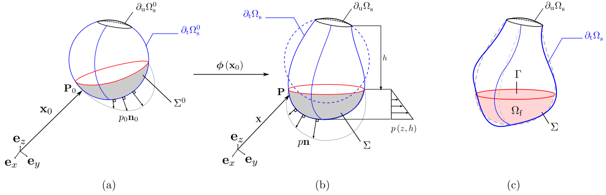
Figure 1: (a) Reference configuration of the internal surface of a tank ; (b) Current configuration of internal surface of a tank loaded by hydrostatic follower forces; (c) Linearized hydroelastic vibration around a pre-stressed state without gravity effects
