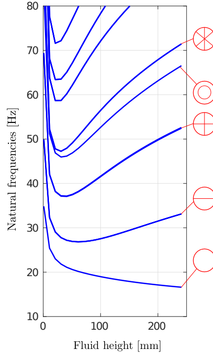
Figure 6: Evolution of natural frequencies in function of the fluid height with \mathbf{K}_{\text{tan}} = \mathbf{K}_{\text{mat}} + \mathbf{K}_{\text{geo}} - \mathbf{K}_{\text{fol}}
