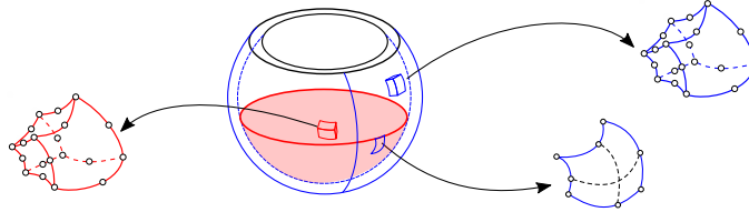
Figure 3: FE discretization with twenty nodes quadratic volumetric element (HEXA 20) for the solid and fluid domains and height nodes quadratic surfacic elements (QUAD 20) for surfacic domains. The fluid and the solid domains have coincident meshes.
