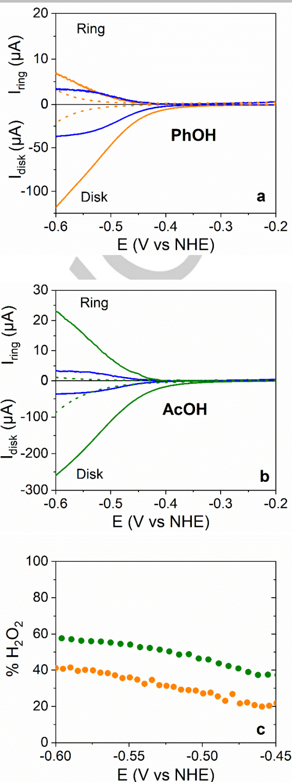
Figure 5. (a, b). Rotating ring-disk electrodes (RRDE) voltammograms under O_2 -saturated atmosphere in DMF (0.1 M nBu_4NPF_6 ) on GC electrode ( \varnothing 5 mm), scan rate 10 mV \cdot s^{-1} , 500 rpm, ring current recorded with Pt ring held at 1.07 V vs NHE. All blue curves are for CuL (1 M), a). CuL (1 M) + PhOH (50 mM, orange trace) and b). CuL (1 M) + AcOH (50 mM, green trace). The RRDE voltammograms of acids in the absence of CuL are shown as dashed line for comparison. In the orange and green plain curves, I_{ring} has been corrected by subtracting of the value measured without acid. (c). The RRDE-determined % of produced H_2O_2 for reduction of one molecule of O_2 vs applied potential for the two different acids (same color code).
