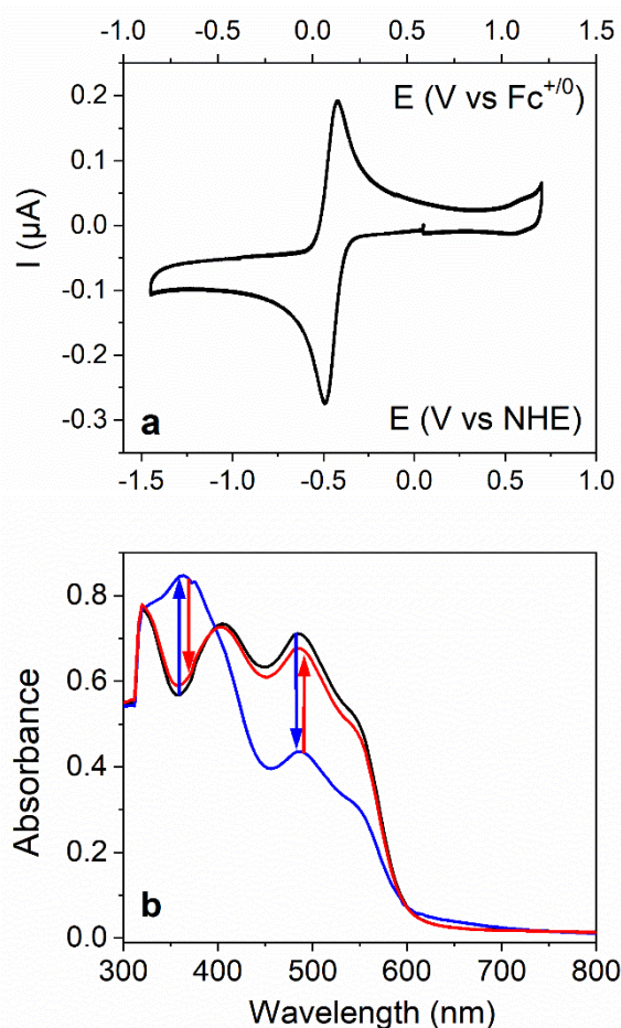
Figure 2. a). Cyclic voltammogram of CuL (1 mM) recorded under Ar-saturated DMF (0.1 M n Bu 4 NPF 6 ), on GC electrode ( \phi 1.6 mm), scan rate 100 mV·s –1 ; b). Electronic absorption spectra for the neutral CuL (black line), one-electron-reduced species CuL – (blue line) and electrochemically re-oxidized CuL (red line).
