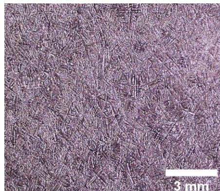
Fig. 4 Solidified melt Pb:Sn in ratio 60:40 ((POK40).
