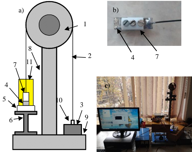
Fig. 1 Experimental setup: a) schematic presentation of the measuring unit: 1-pulley, 2-non-expanding string, 3-balance scale, 4-Wilhelmy plate, 5-oven, 6- Z-axis movable table, 7-Wilhelmy plate holder, 8, 9-support of the system, 10-weight, 11- isolating container; b) picture of Wilhelmy plate with the holder; c) picture of the entire setup including the controllers and the computer.
