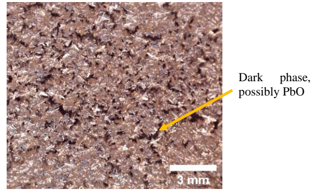
Fig. 3 Solidified melt Pb:Sn in ratio40:60 (POK60).
