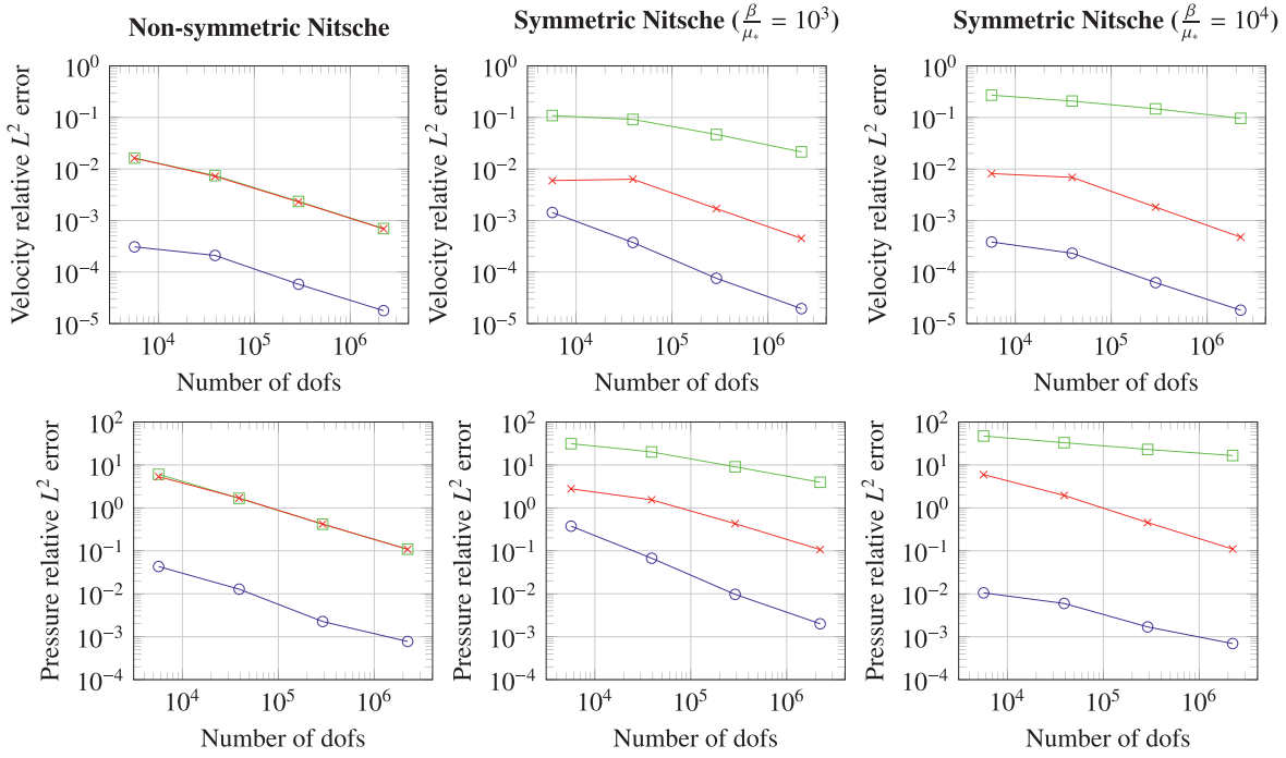
Fig. 5. Convergence comparison, Navier's slip with \theta = 0.5 - different normals: \text{---}\circ\text{---} \mathbf{n}_h^a \text{---}\square\text{---} \mathbf{n}_h^f \text{---}\times\text{---} \mathbf{n}_h^v
