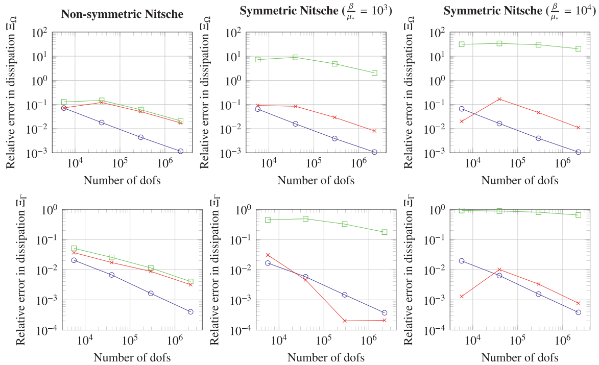
Fig. 6. Convergence comparison, Navier's slip with \theta = 0.5 - different normals: \text{---}\circ\text{---} \mathbf{n}_h^a \text{---}\square\text{---} \mathbf{n}_h^f \text{---}\times\text{---} \mathbf{n}_h^v
