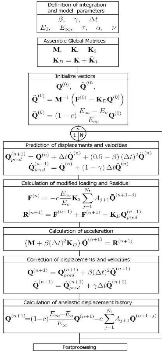
Figure 4: Flow-chart of the modified Newmark method.
