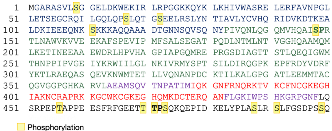
Figure 4. Phosphorylated residues in HIV-1 Pr55 Gag . The different colors represent the Pr55 Gag domains, MA (blue), CA (green), spacer peptides p1 and p2 (purple), NC (red), and p6 (black). Phosphorylation positions are highlighted in yellow. TP (in p6) and SP (in CA) motifs involved in the ERK2 recruitment and incorporation into viral particle are indicated in bold [91,93–96].
