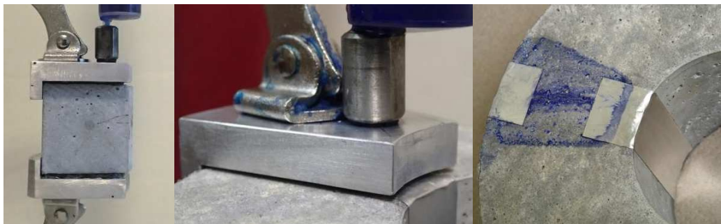
153 Fig. 1. From left to right – cross-sectional view of the injection device setup on a mortar sample; 154 upper side view; cracked mortar sample after injection of a colored solution
