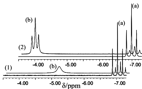
Figure 1. 1 H NMR (500 MHz) spectra in THF- d 8 (1) or CD 2 Cl 2 (2) of: (a) compound 1 alone; (b) compound 1 in the presence of slightly less than 1 equiv of Et 2 O·HBF 4 . [1] = 0.04 M; T = 200 K.
