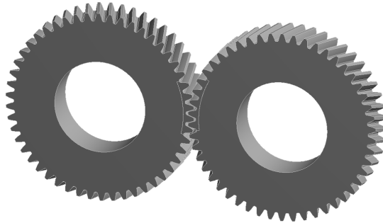
Figure 10: Helical gear pair without and with longitudinal crowning
