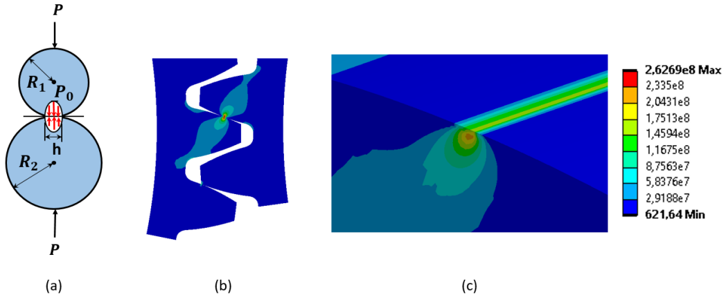
Figure 9: (a) Description of the cylindrical contact stress claimed by Hertz theory, (b) shear stress for a torque of T = 100 N.m and (c) a close-up of the shear stress in Pa at the middle of the tooth width is depicted.
