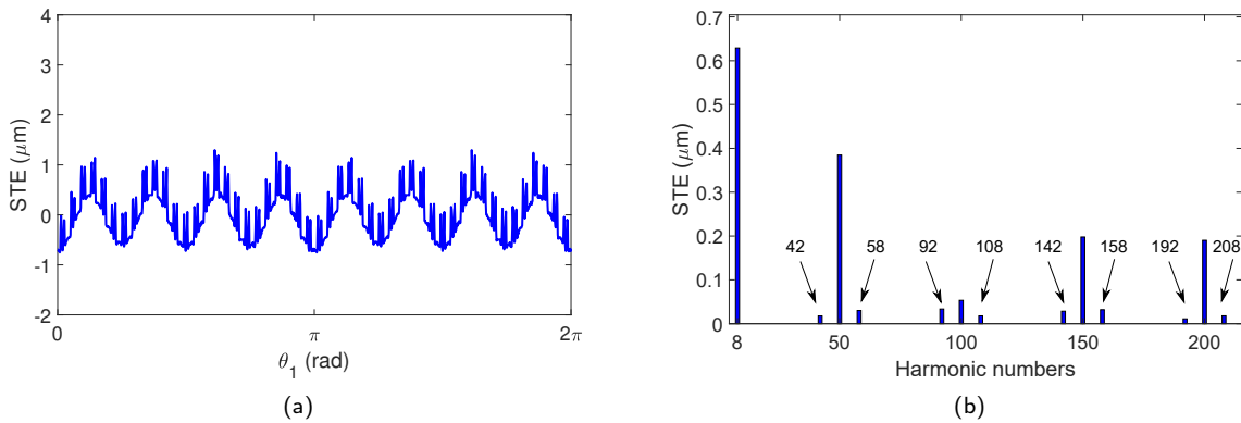
Figure 16: Fluctuation of the static transmission error of the gear pair with holes (a) and frequency spectrum (b) for an output torque T = 115 \text{ N.m}
