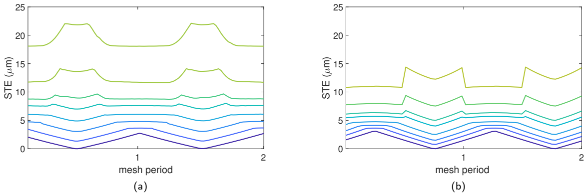
Figure 5: The static transmission error for different torque levels T = [0.5, 15, 30, 50, 80, 100, 150, 250] N.m and over two mesh periods. Numerical results through ANSYS Mechanical (®) solver (a) and the classical method (b).
