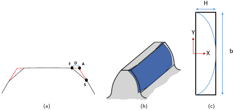
Figure 2: Description of linear tip relief deviation (a) where S is the starting point, D is an amount of profile modification at the tooth tip starting for the point A to the point F . Longitudinal crowning modification (b) and parameters description from the top (c). H is the maximum depth of crowning. y is the varying depth parameter covering the tooth width b .
