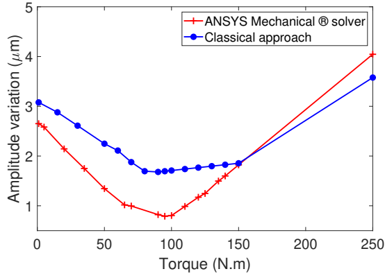
Figure 7: Comparison of the different peak to peak transmission error (a): — Classical approach, and — ANSYS Mechanical solver
