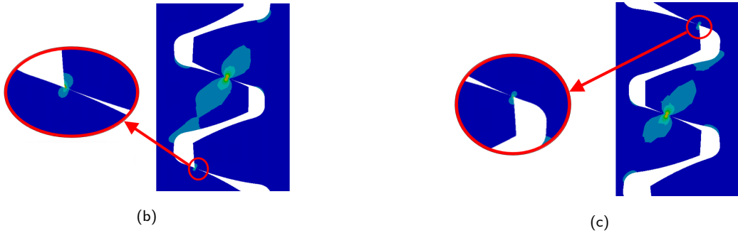
Figure 6: STE for 150 N.m with two contact positions named POS1 and POS2 (a). A close-up at the contact POS1 (b) and POS2 (c).
