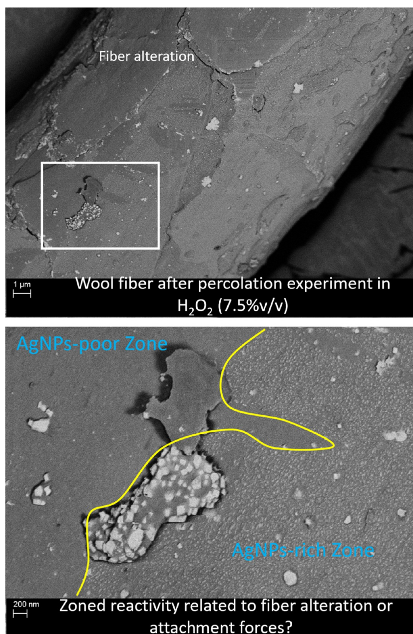
Figure 8. FESEM images at two different magnifications showing sheep's wool fiber after flow-through reactor experiment with oxygenated water (7.5% v/v). The high concentration of Ag-NPs remains still adhered onto fiber despite the surface fiber alteration.
