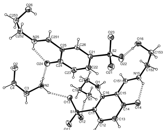
Figure 3. An ORTEP view of the asymmetric unit in the structure of [\text{HOCH}_2\text{CH}_2\text{NH}_3][\text{H}_2\text{SAE}] . Ellipsoids are shown at the 30% probability level. For Anion 1, only one of the two disordered tautomeric forms is shown (see Experimental).
