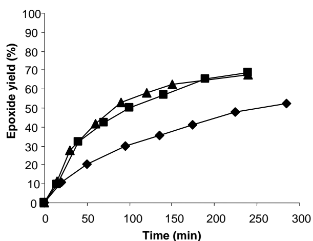
Figure 5. Comparison of the catalysts 3 (triangles), 4 (diamonds) and 5 (squares) in cyclooctene epoxidation in [BMIM][NTf 2 ].
