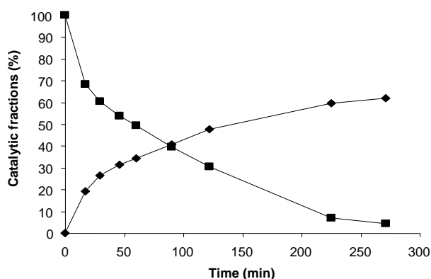
Figure 6: Kinetic profile for cyclooctene epoxidation with catalyst 3 in [BMIM][NTf 2 ]. Squares: cyclooctene residual fraction; diamonds: cyclooctene oxide yield.
