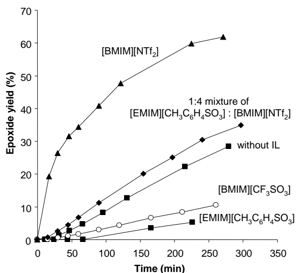
Figure 4. Comparison of the catalytic activity of 3 in different IL media.
