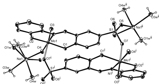
Figure 1. An ORTEP view of the molecular structure of compound 3 . The ellipsoids are shown at the 30% probability level.
