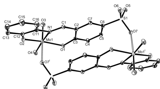
Figure 1. An ORTEP view of the molecular structure of compound 3 . The ellipsoids are shown at the 30% probability level.
