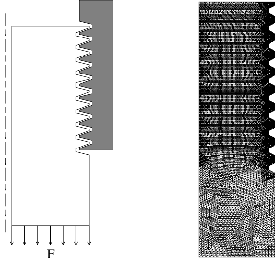
Figure 20: Geometry and mesh of the screw-press
