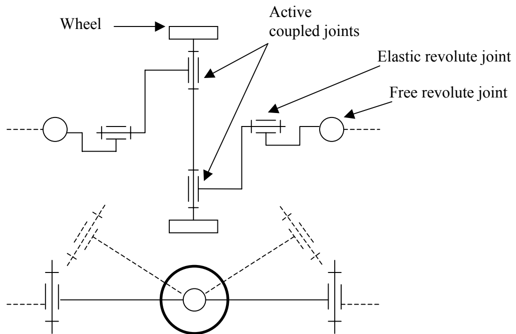
Fig. 2: Module kinematics (top view and side view)
